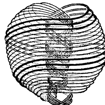
The pulsating Anu or ultimate Physical Atom.
