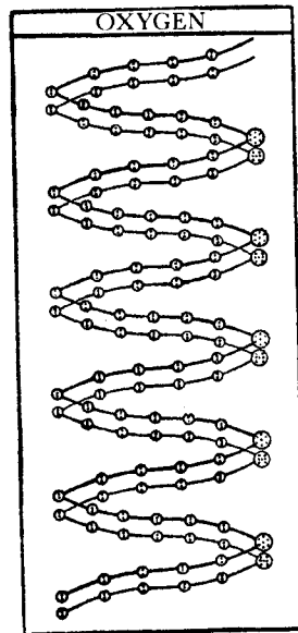
THE OXYGEN MOLECULE showing vitality globules linked to the double helix (on the right).
