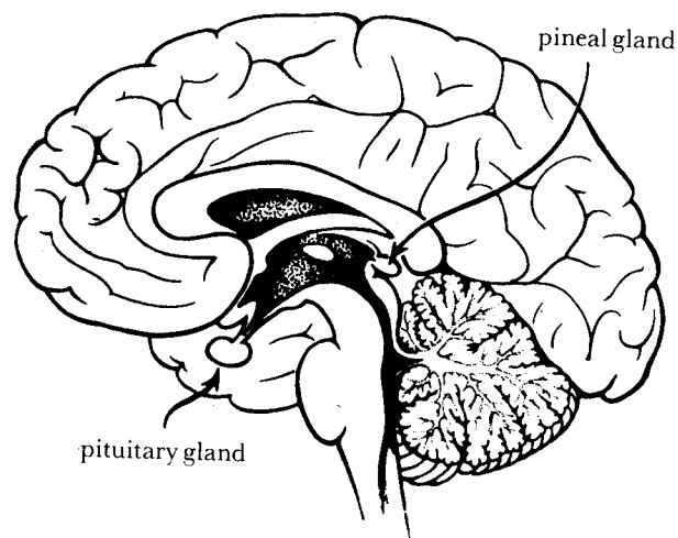
HEMISECTED BRAIN
