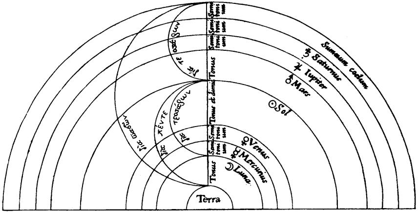
FIGURE 13. THE MUSIC OF THE SPHERES
